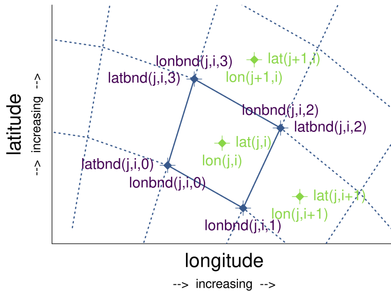
Figure 7.2. Order of \text{lonbnd}(j,i,0) to \text{lonbnd}(j,i,3) and of \text{latbnd}(j,i,0) and \text{latbnd}(j,i,3) in the case of two-dimensional horizontal coordinate axes. Tuples (\text{lon}(j,i), \text{lat}(j,i)) represent grid cell centers and tuples (\text{lonbnd}(j,i,n), \text{latbnd}(j,i,n)) represent the grid cell vertices.
