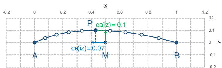
Figure J.4. With the expansion coefficient c_e > 0 and the alignment coefficient c_a > 0 , the method reconstitutes the points at intervals of expanding size ( c_e ) along an arc with an alignment offset ( c_a ) from the great circle between tie points A and B.
