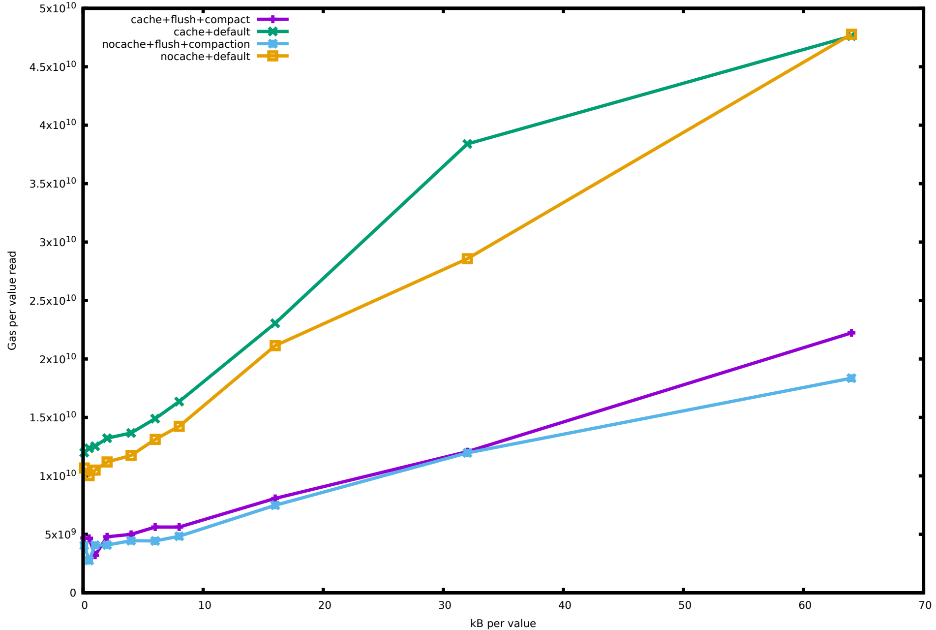
RocksDB worst-case read performance (All unique keys)
