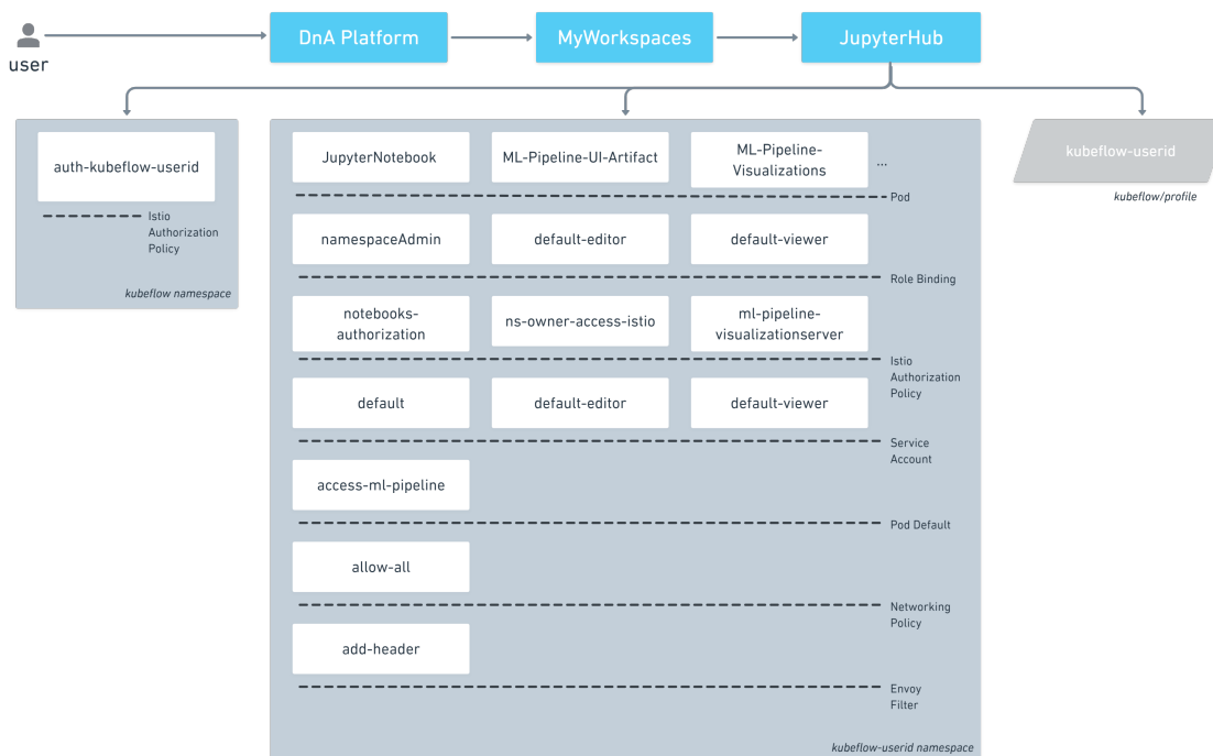
Figure 5.6: Architecture of the KFP profile generation process
