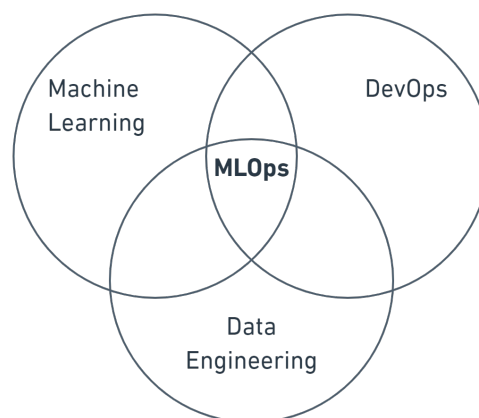
Figure 3.4: MLOps
