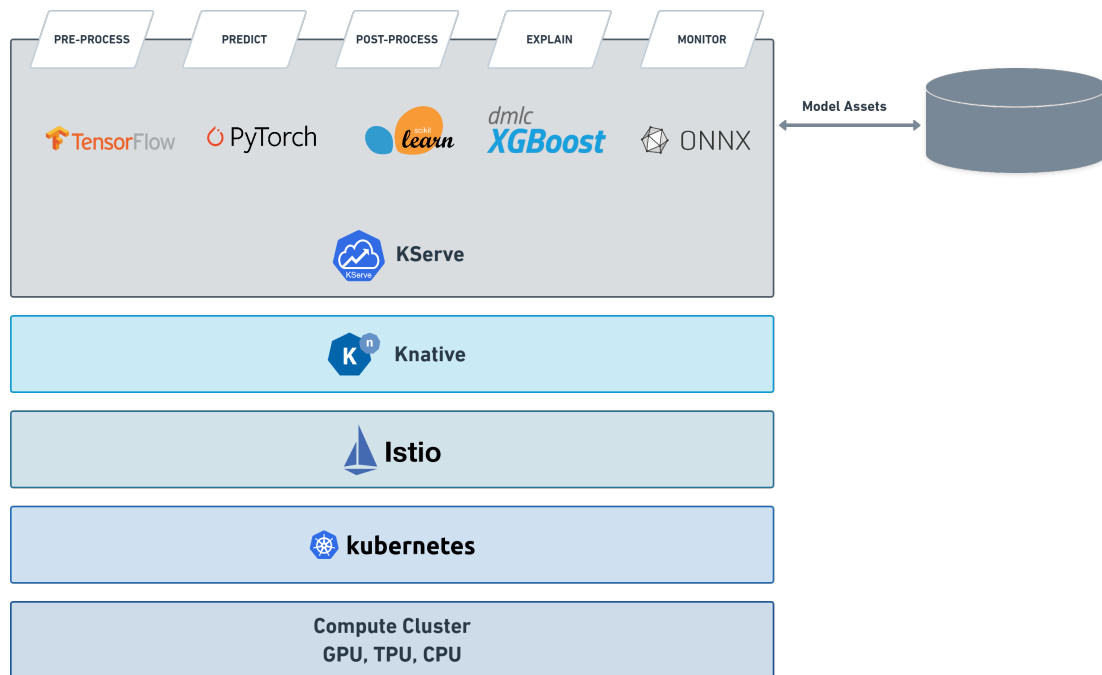
Figure 3.10: The architecture of KServe (Patterson et al., 2021)
