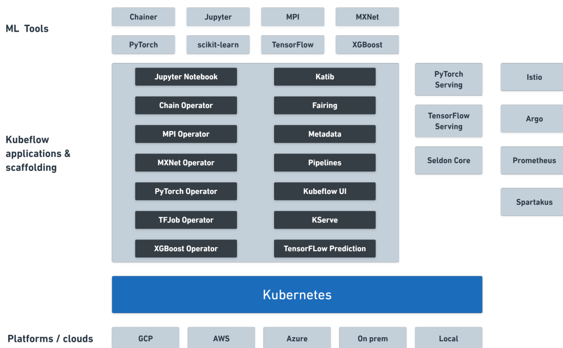
Figure 3.8: The components of Kubeflow (Kubeflow, 2021a)
