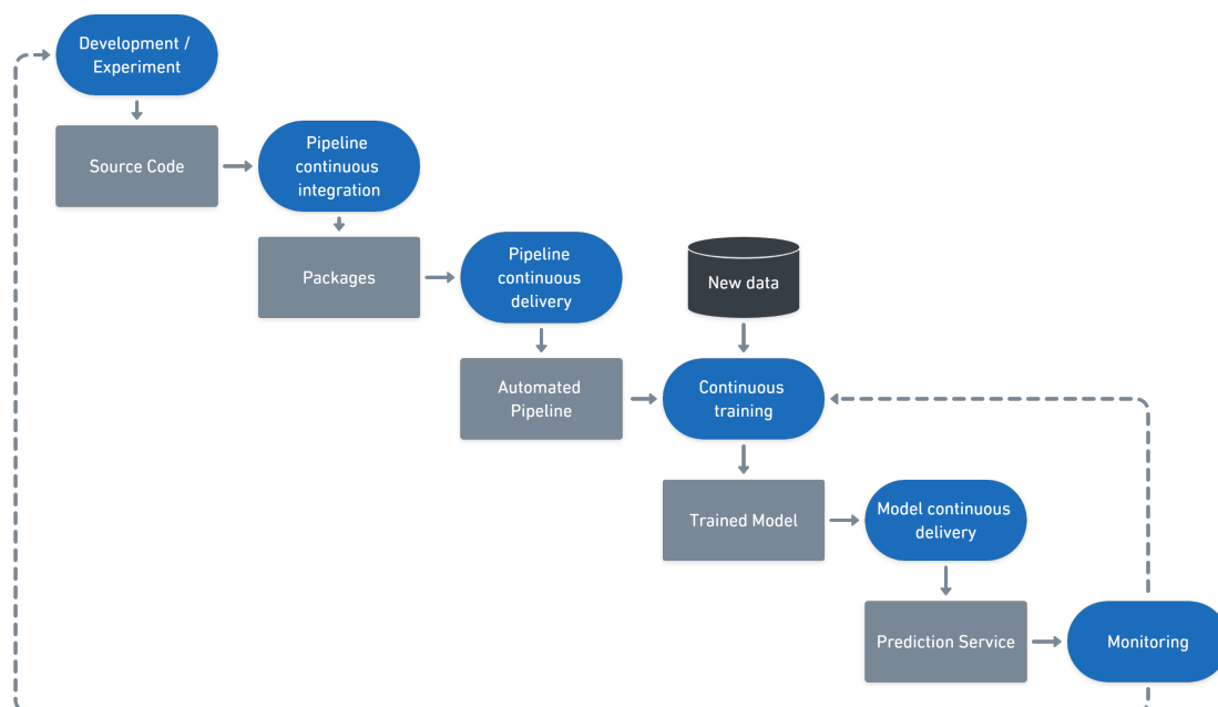
Figure 4.1: The 5 stages for MLOps by Google (2020)
