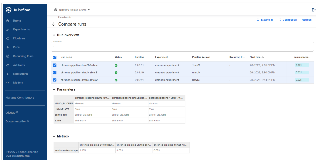
Figure 6.7: Comparing different KF pipeline versions
