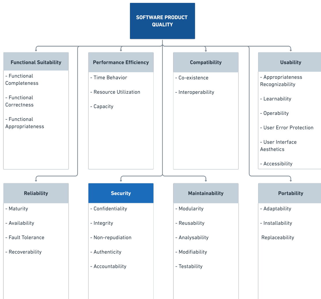
Figure 5.13: The Software Product Quality Model (ISO/IEC 25010, 2011)
