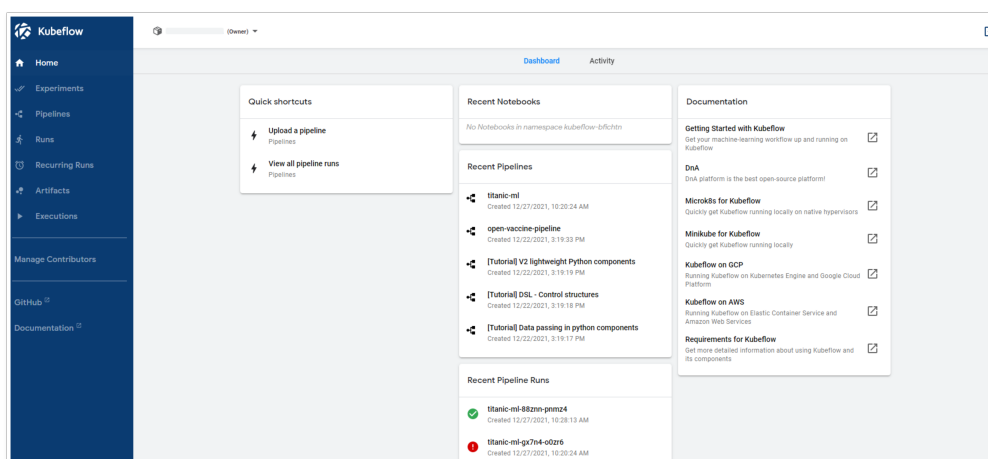
Figure 5.2: Example of the Kubeflow Dashboard
