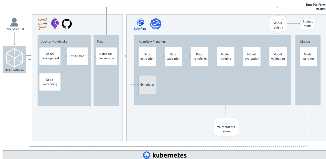
Figure 4.2: The MLOps Workflow for the DnA Platform
