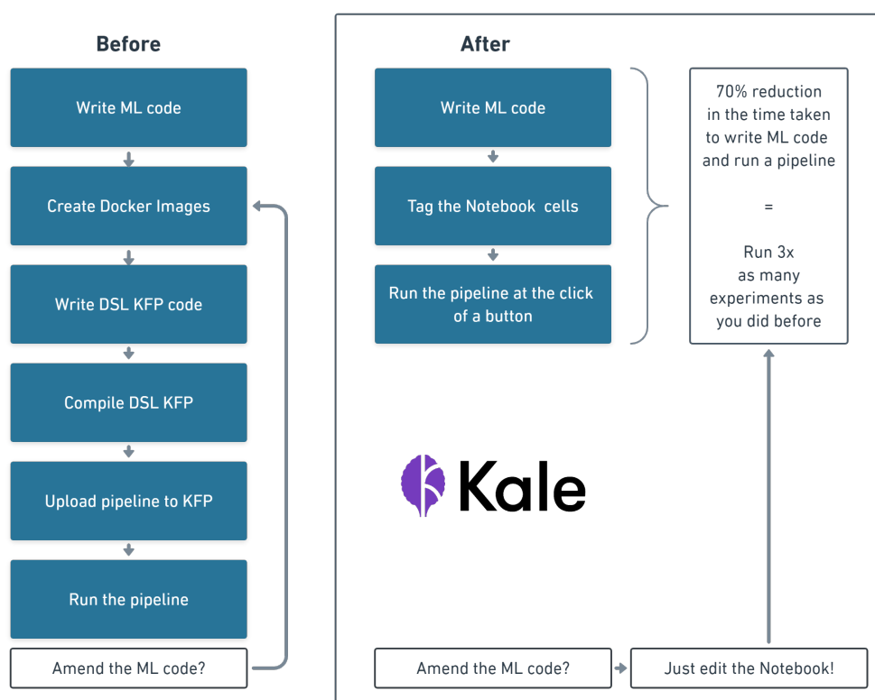
Figure 3.9: Kale reduces the steps for the creation of a Kubeflow Pipeline (Fioravanzo & Koukis, 2020)
