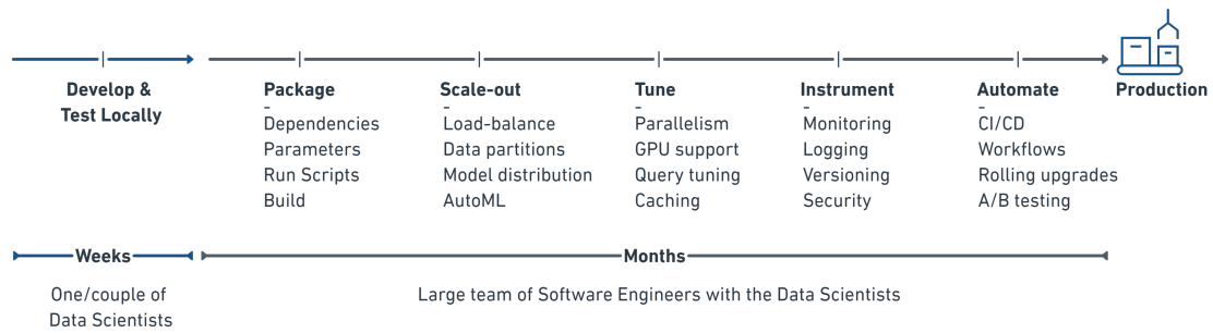
Figure 2.1: ML models from Lab to Production (Haviv, 2020)
