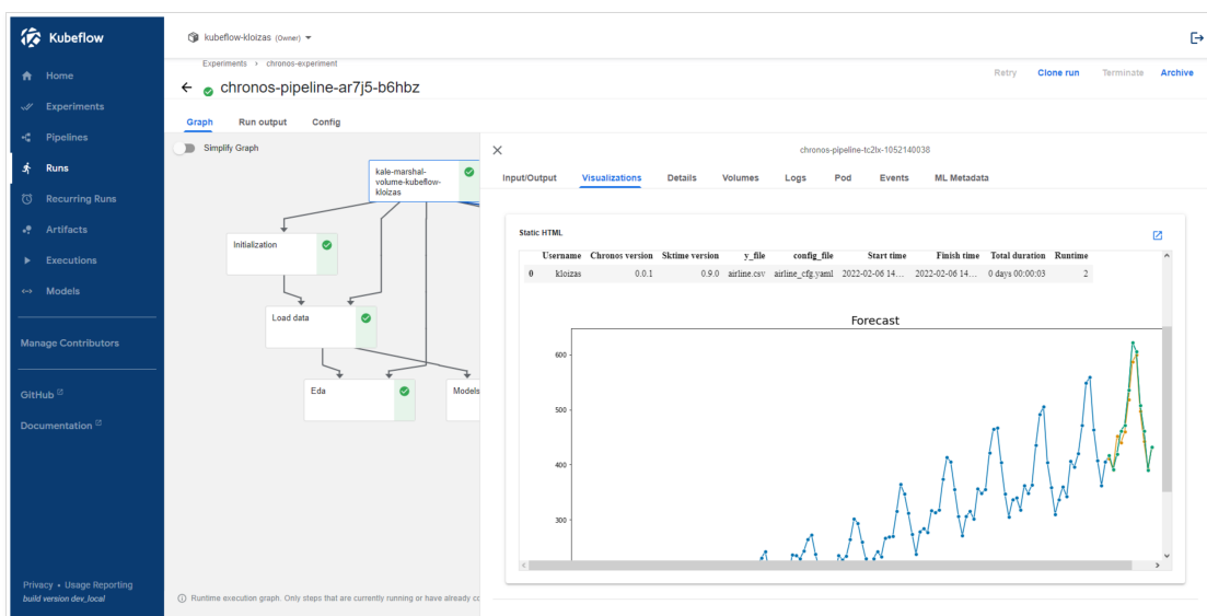
Figure 6.6: A visualization example from a KFP step
