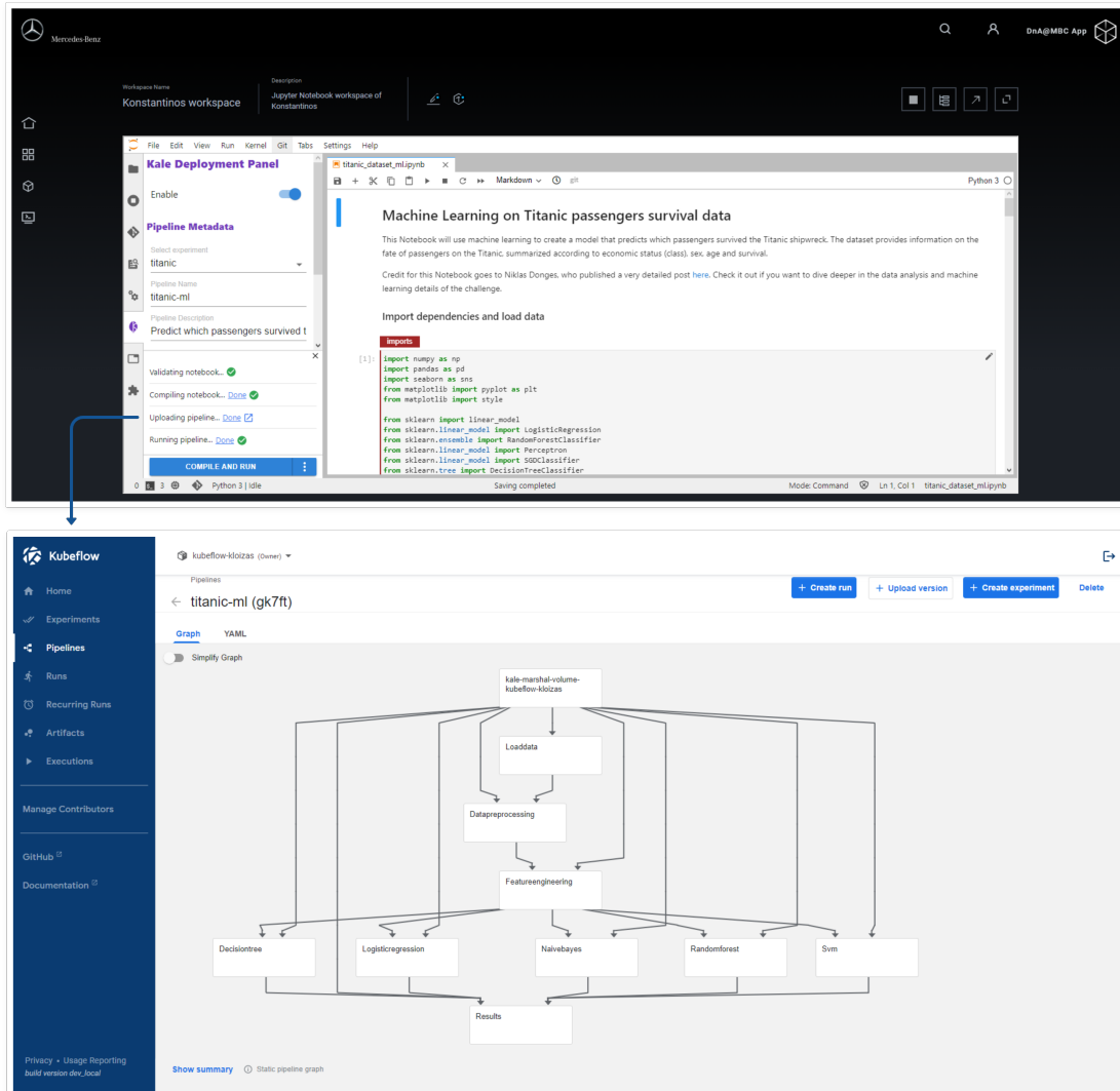
Figure 5.7: Kale generates hyperlinks to access the KFP UI
