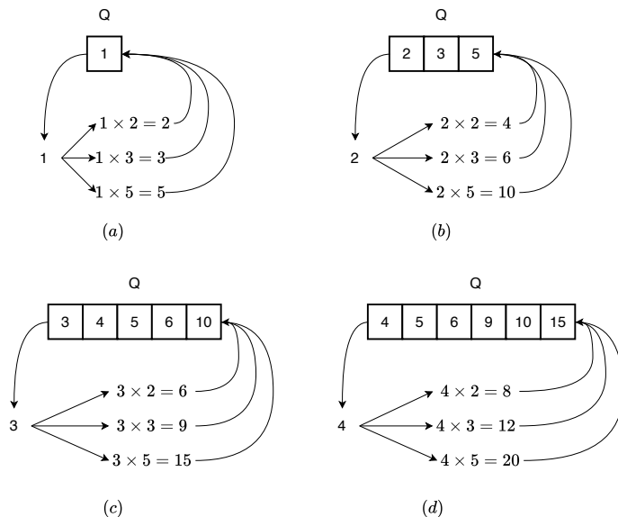
Figure 2: First 4 steps: add 1; add 2, 3, 5; add 4, 6, 10; add 9, 15, drop 6.
