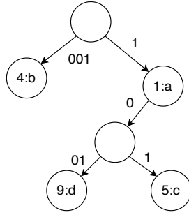
Figure 6.4: Little endian integer tree for the map \{1 \rightarrow a, 4 \rightarrow b, 5 \rightarrow c, 9 \rightarrow d\} .
