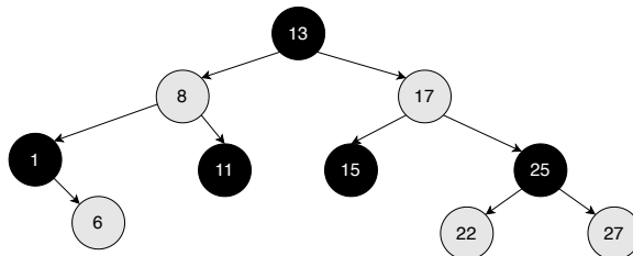
Figure 4.5: Hide the NIL nodes
