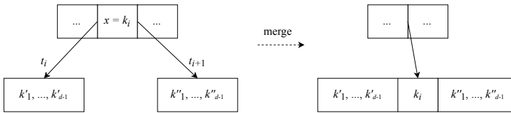
Figure 7.14: Merge before delete
