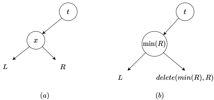
Figure 2.6: Delete a branch with two none empty sub-trees.
