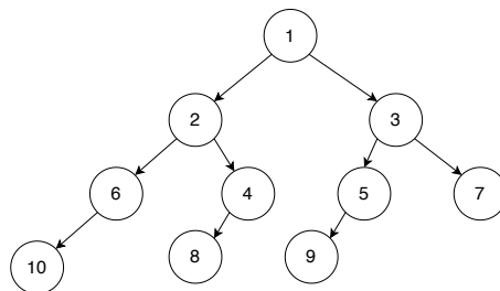
Figure 8.9: Skew tree built from [1, 2, \dots, 10] .
