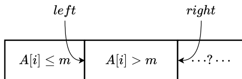
Figure 1: All A[i] \leq m where 0 \leq i < left ; while A[i] > m where left \leq i < right . The rest elements are yet to be scanned.
