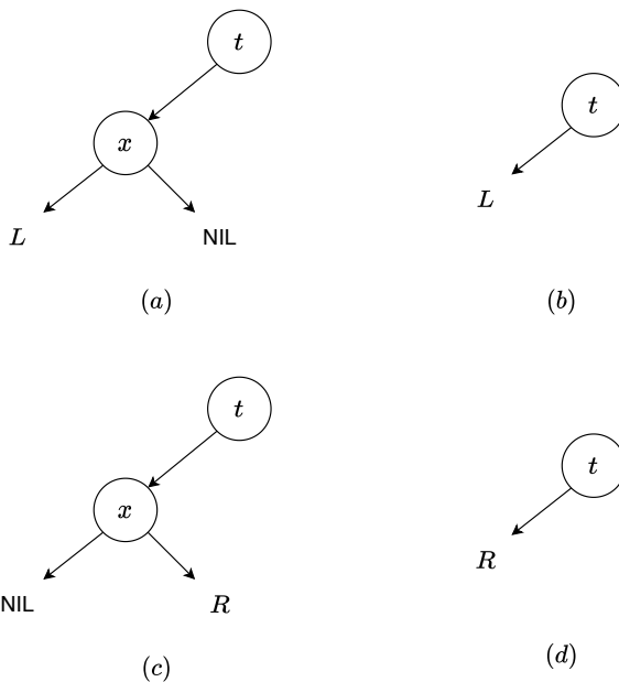
Figure 2.5: Delete a node with only a none empty sub-tree.
