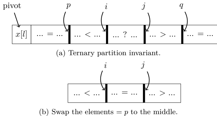
Figure 13.4: Ternary partition
