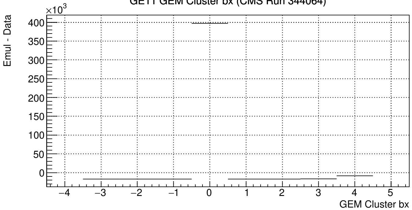
GE11 GEM Cluster bx (CMS Run 344064)
