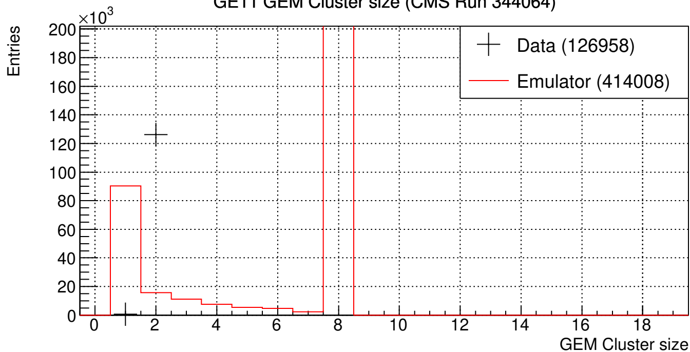
GE11 GEM Cluster size (CMS Run 344064)
