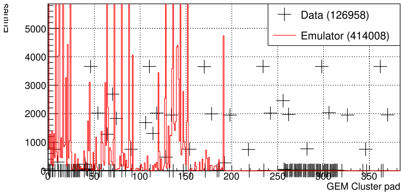
GE11 GEM Cluster pad (CMS Run 344064)
