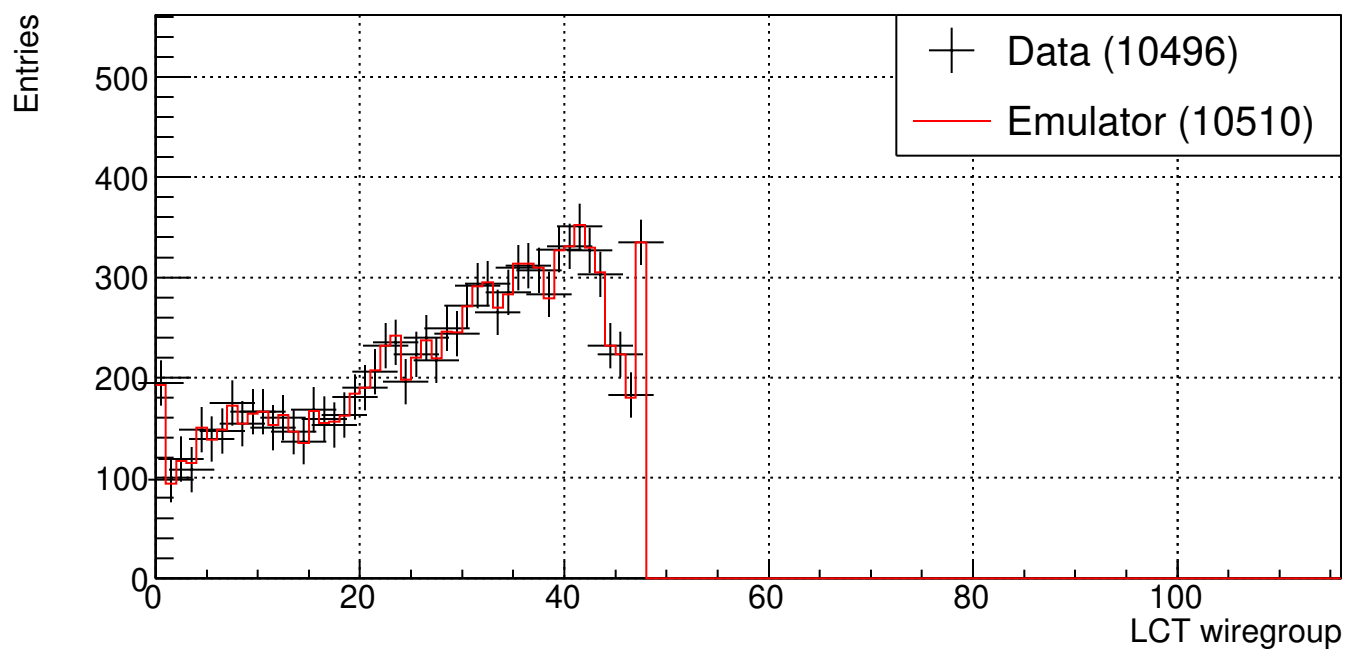
ME11 LCT wiregroup (B904 Cosmic Run 210609_142357)
