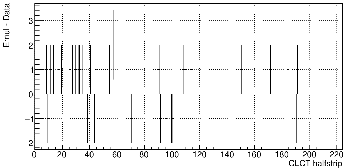
ME11 CLCT halfstrip (B904 Cosmic Run 210609_142357)
