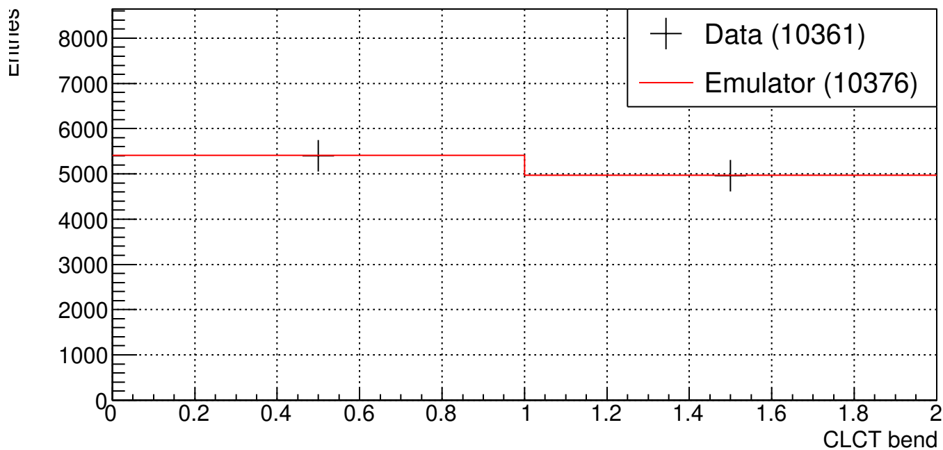
ME11 CLCT bend (B904 Cosmic Run 210609_142357)
