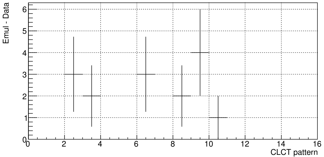
ME11 CLCT pattern (B904 Cosmic Run 210609_142357)
