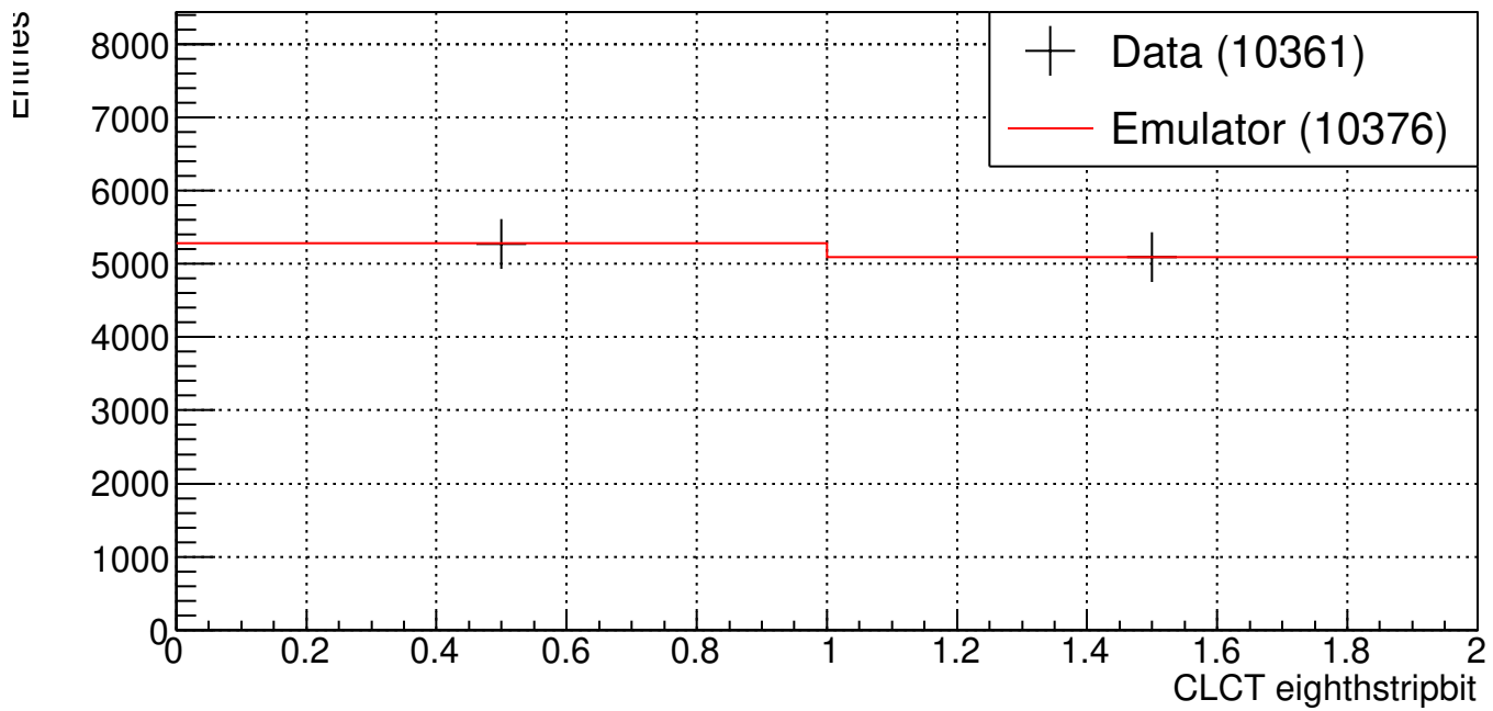
ME11 CLCT eighthstripbit (B904 Cosmic Run 210609_142357)
