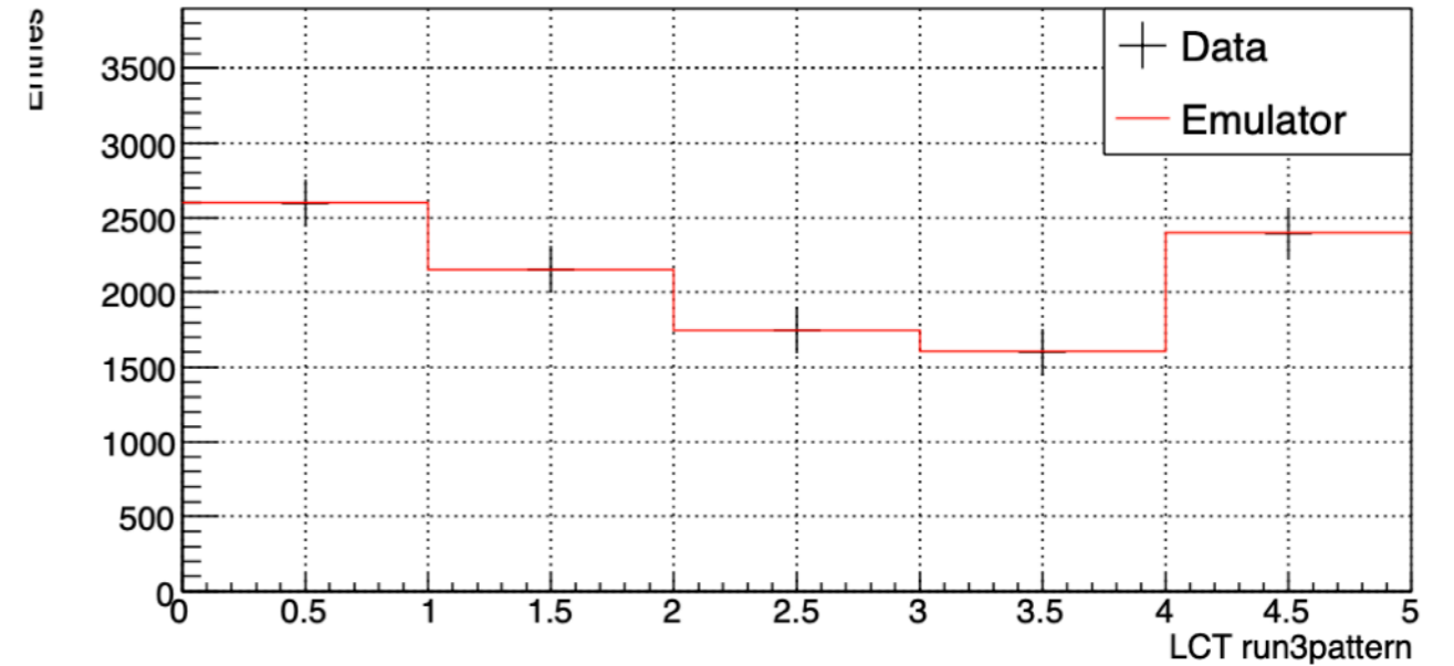
ME11 LCT run3pattern (B904 Cosmic Run 210609_142357)
