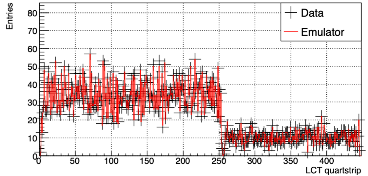
ME11 LCT quartstrip (B904 Cosmic Run 210609_142357)
