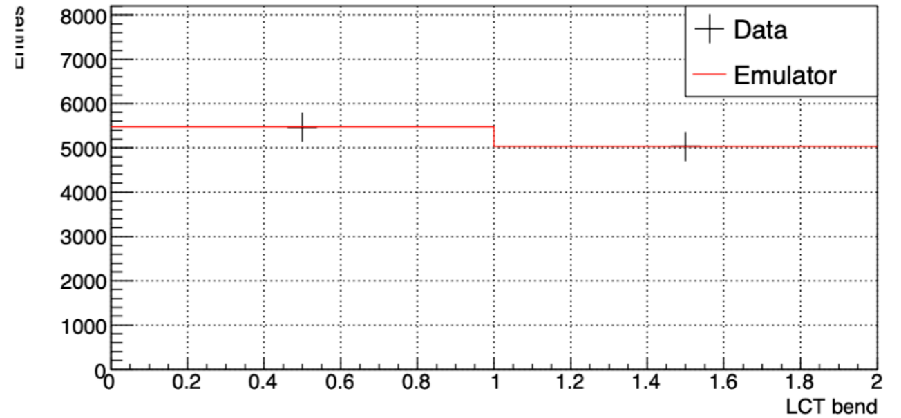
ME11 LCT bend (B904 Cosmic Run 210609_142357)
