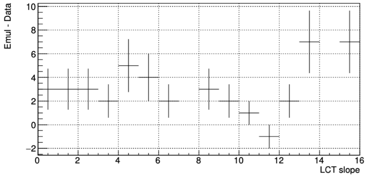
ME11 LCT slope (B904 Cosmic Run 210609_142357)
