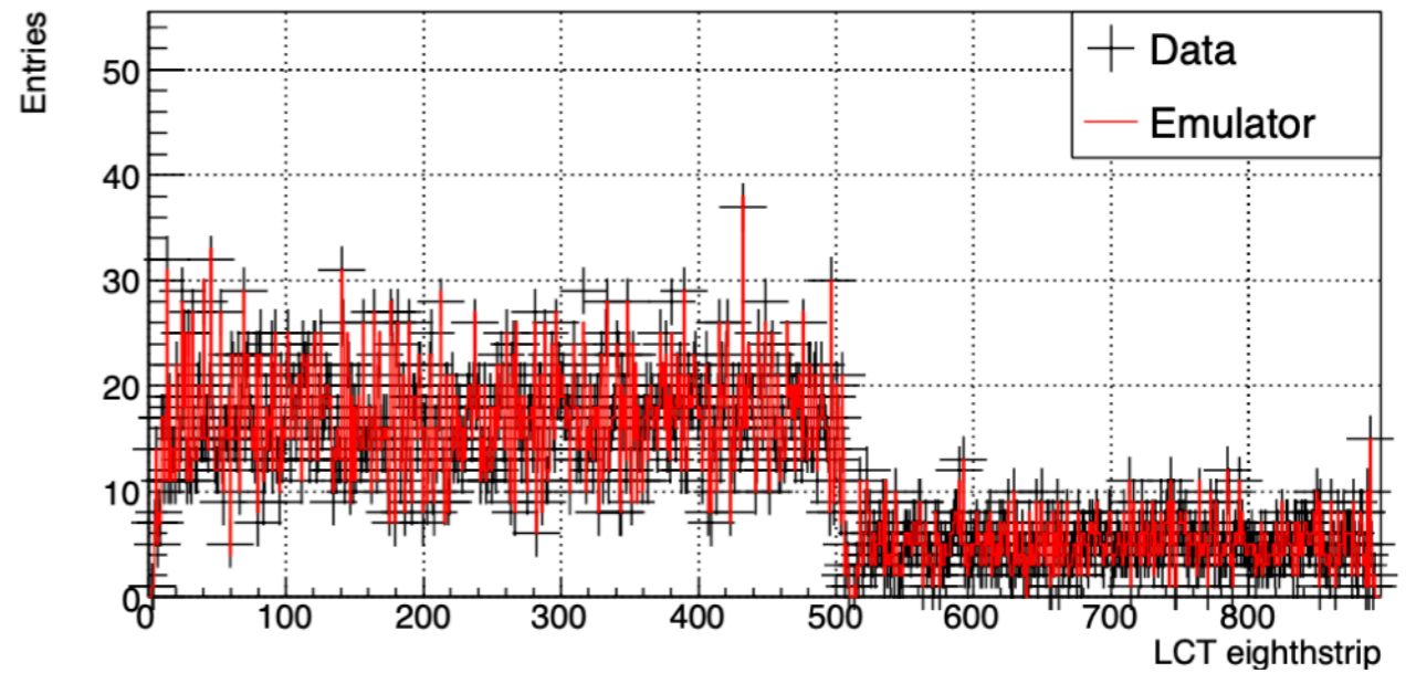
ME11 LCT eighthstrip (B904 Cosmic Run 210609_142357)
