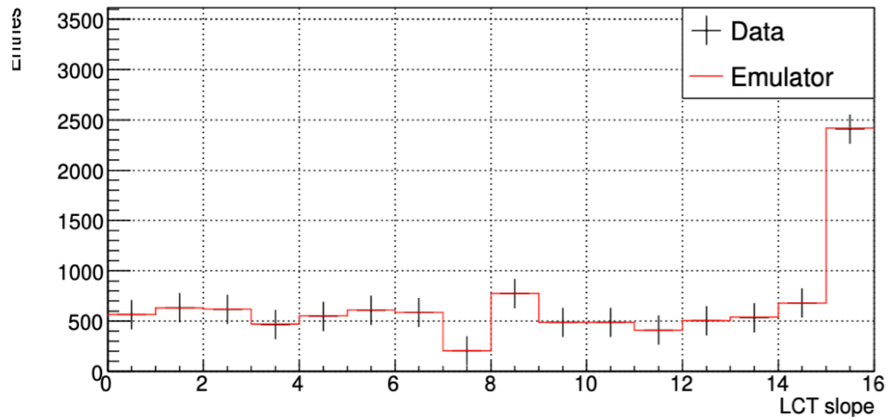
ME11 LCT slope (B904 Cosmic Run 210609_142357)
