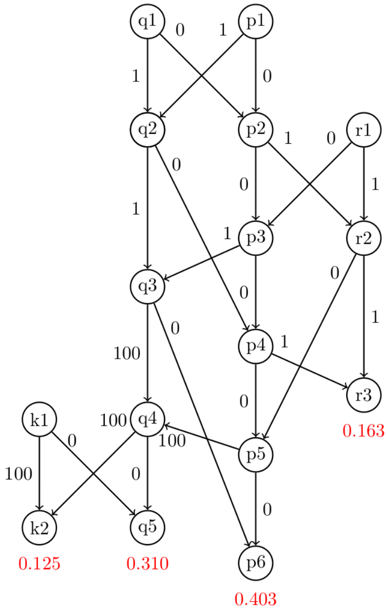
Figure 3.3: NetFlow algorithm
