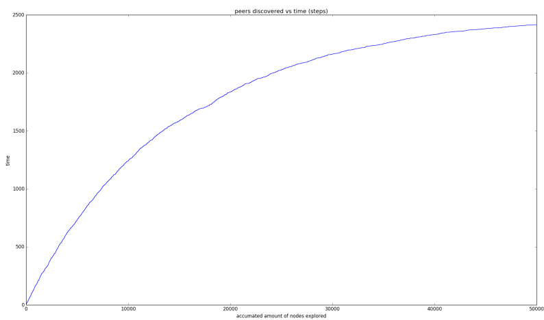
Figure 5.6: Bias Random Walker Peer Discovery
