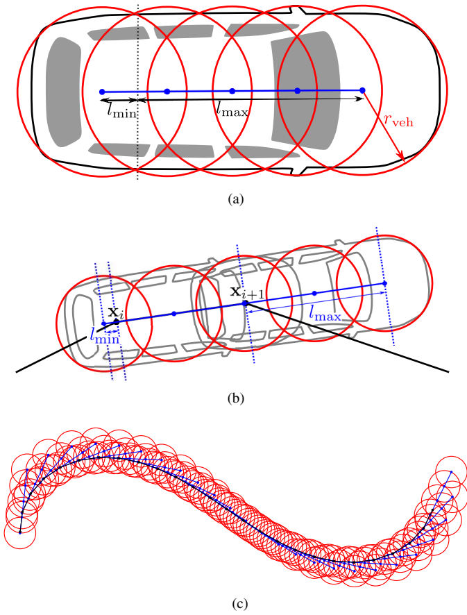
Figure 3: Circle decomposition of vehicle shape and maneuver area
